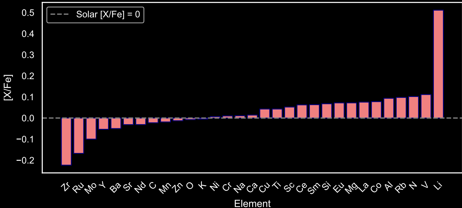
Abundance Pattern for GALAH Main Sequence Stars: Star Field [63] (N=109)
