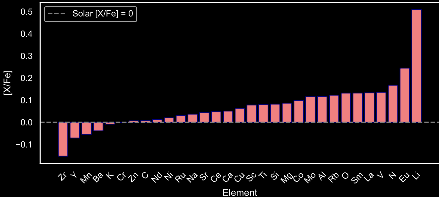
Abundance Pattern for GALAH Star Field [63] (N=243)
