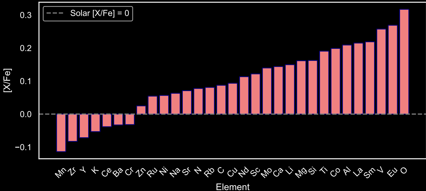
Abundance Pattern for GALAH Red Giants: Star Field [63] (N=57)
